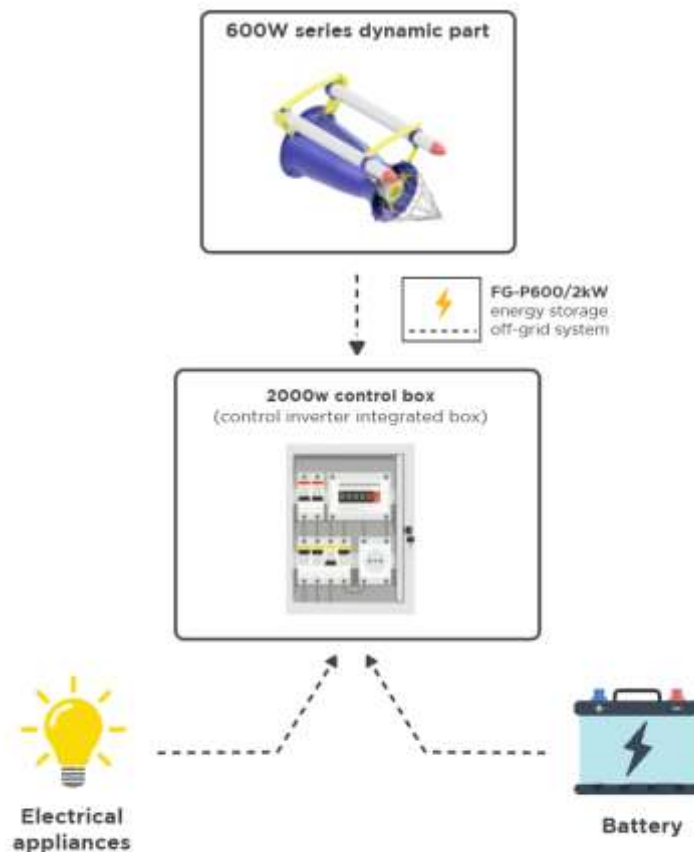
Figure 20 - System setup
