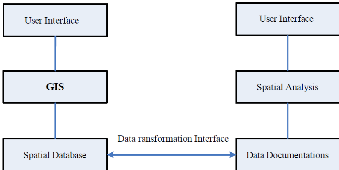
Figure 1 - Loose-coupling of Spatial Analysis and GIS
